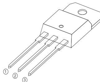
TO-220A Insulated
