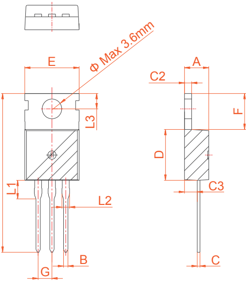
TO-220C
