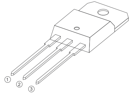
TO-220A Insulated
